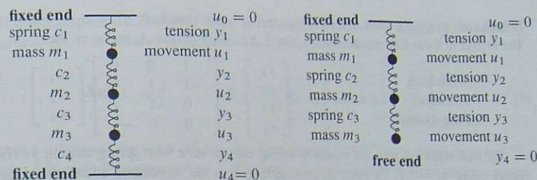
Figure 8.1: Lines of springs and masses: fixed-fixed and fixed-free ends.
