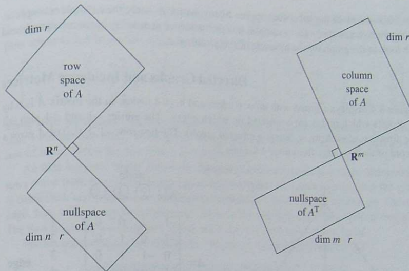
Figure 8.3: Big picture: The four subspaces with their dimensions and orthogonality.
