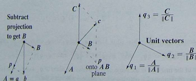
Figure 4.11: First project b onto the line through a and find the orthogonal B as b - p . Then project c onto the AB plane and find C as c - p . Divide by \|A\| , \|B\| , \|C\| .
