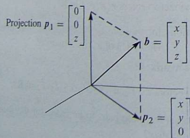
Figure 4.4: The projections \mathbf{p}_1 = P_1 \mathbf{b} and \mathbf{p}_2 = P_2 \mathbf{b} onto the z axis and the xy plane.
