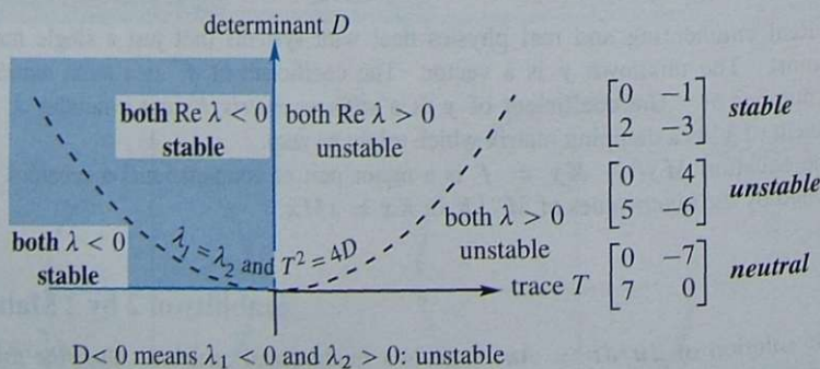
Figure 6.5: A 2 by 2 matrix is stable ( u(t) \rightarrow 0 ) when trace < 0 and det > 0 .
