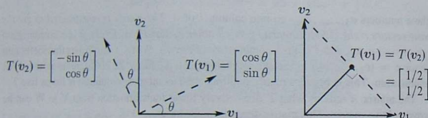
Figure 7.3: Two transformations: Rotation by \theta and projection onto the 45^\circ line.
