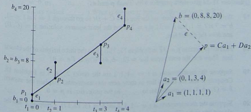
Figure 4.9: Problems 1–11: The closest line C + Dt matches Ca_1 + Da_2 in \mathbb{R}^4 .
