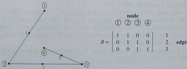
Figure 8.4b: Tree with 3 edges and 4 nodes and no loops.
