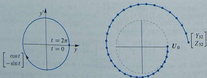
Figure 6.3: Exact u = (\cos t, -\sin t) on a circle. Forward Euler spirals out (32 steps).
