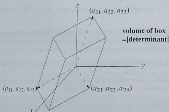
Figure 5.4: Three-dimensional box formed from the three rows of A .
