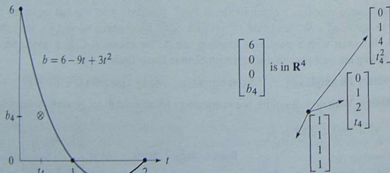
Figure 4.8: From Example 3: An exact fit of the parabola at t = 0, 1, 2 means that p = b and e = 0 . The point b_4 off the parabola makes m > n and we need least squares.
