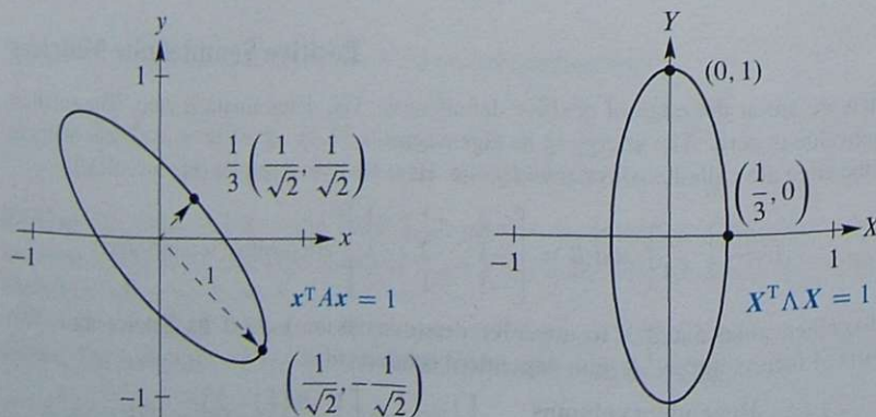
Figure 6.7: The tilted ellipse 5x^2 + 8xy + 5y^2 = 1 . Lined up it is 9X^2 + Y^2 = 1 .
