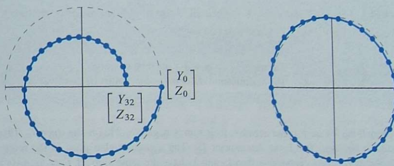
Figure 6.4: Backward differences spiral in. Leapfrog stays near the circle Y_n^2 + Z_n^2 = 1 .
