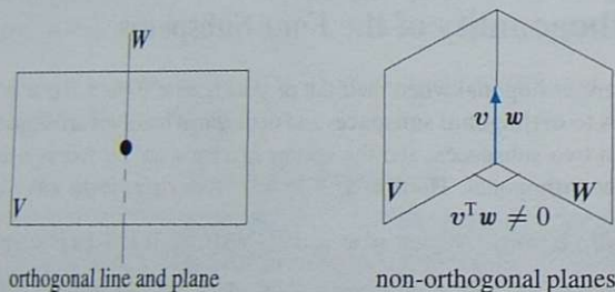
Figure 4.1: Orthogonality is impossible when \dim V + \dim W > \text{dimension of whole space} .
