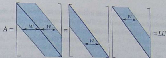
Figure 9.1: A = LU for a band matrix. Good zeros in A stay zero in L and U .
