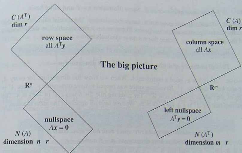
Figure 3.5: The dimensions of the Four Fundamental Subspaces (for R and for A ).
