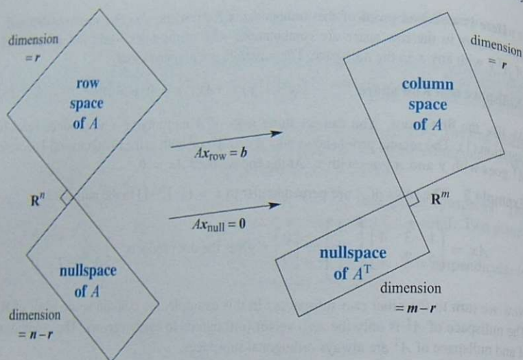
Figure 4.2: Two pairs of orthogonal subspaces. The dimensions add to n and add to m . This is an important picture —one pair of subspaces is in \mathbb{R}^n and one pair is in \mathbb{R}^m .
