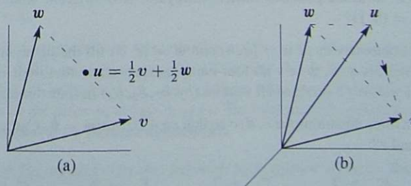
Figure 1.5: Problems 15–19 in a plane
