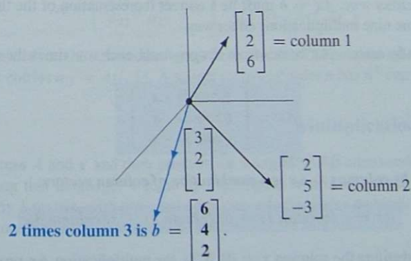
Figure 2.4: Column picture: (x, y, z) = (0, 0, 2) because 2(3, 2, 1) = (6, 4, 2) = b .
