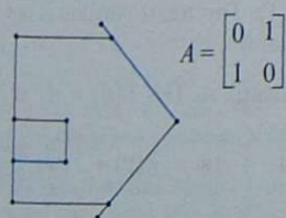
Figure 7.2: Linear transformations of a house drawn by plot2d(A * H) .
