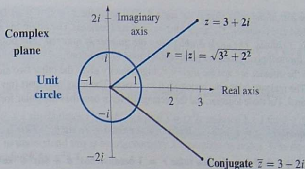
Figure 10.1: The number z = a + bi corresponds to the point (a, b) and the vector \begin{bmatrix} a \\ b \end{bmatrix} .
