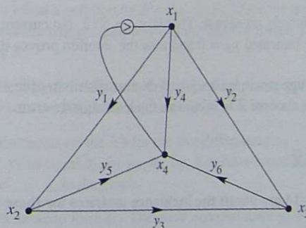
Figure 8.5: The currents in a network with a source S into node 1.
