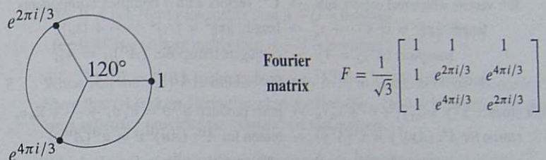
Figure 10.3: The cube roots of 1 go into the Fourier matrix F = F_3 .
