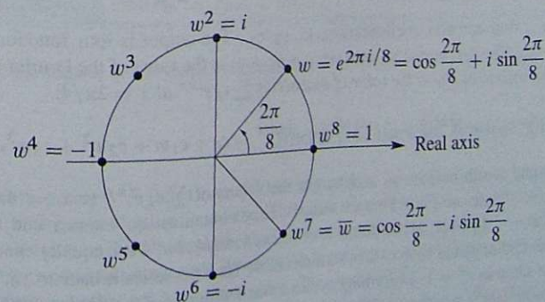
Figure 10.4: The eight solutions to z^8 = 1 are 1, w, w^2, \dots, w^7 with w = (1 + i)/\sqrt{2} .
