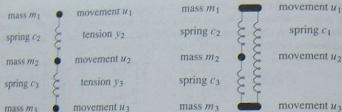
Figure 8.2: Free-free ends: A line of springs and a “circle” of springs: Singular K’s . The masses can move without stretching the springs so Au = 0 has nonzero solutions.
