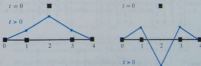
Figure 6.6: Heat diffuses away from box 2 (left). Wave travels from box 2 (right).
