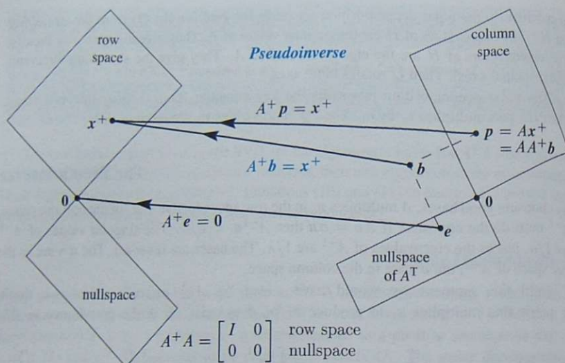
Figure 7.4: Ax^+ in the column space goes back to A^+Ax^+ = x^+ in the row space.
