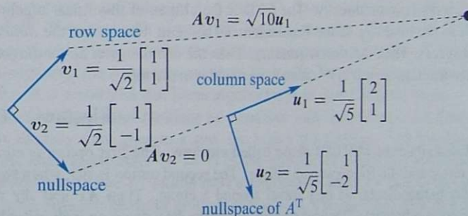
Figure 6.9: The SVD chooses orthonormal bases for 4 subspaces so that Av_i = \sigma_i u_i .
