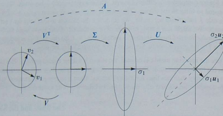
Figure 6.8: U and V are rotations and reflections. \Sigma stretches circle to ellipse.
