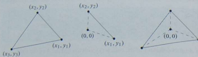
Figure 5.1: General triangle; special triangle from (0, 0) ; general from three specials.
