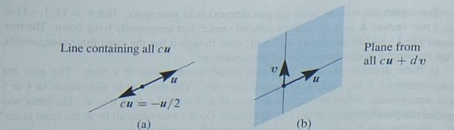
Figure 1.3: (a) Line through u . (b) The plane containing the lines through u and v .
