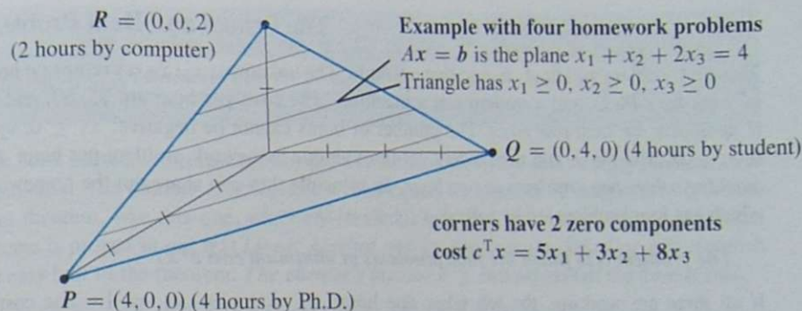
Figure 8.6: The triangle contains all nonnegative solutions: Ax = b and x \geq 0 . The lowest cost solution x^* is a corner P , Q , or R of this feasible set.
