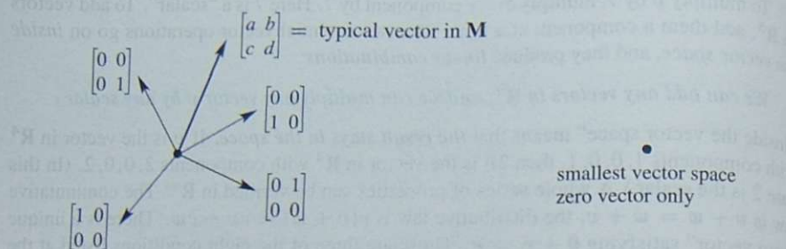
Figure 3.1: “Four-dimensional” matrix space M . The “zero-dimensional” space Z .
