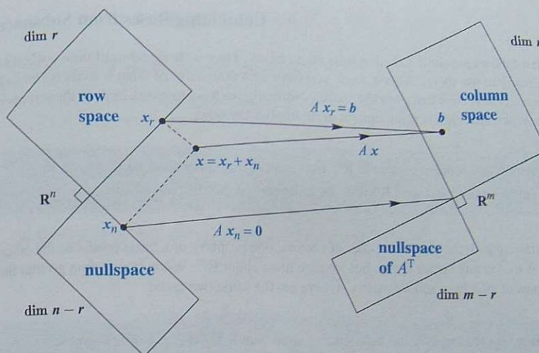
Figure 4.3: This update of Figure 4.2 shows the true action of A on x = x_r + x_n . Row space vector x_r to column space, nullspace vector x_n to zero.
