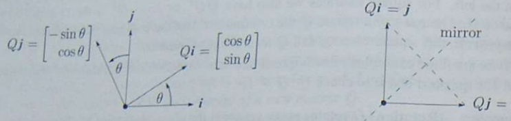
Figure 4.10: Rotation by Q = \begin{bmatrix} c & -s \\ s & c \end{bmatrix} and reflection across 45^\circ by Q = \begin{bmatrix} 0 & 1 \\ 1 & 0 \end{bmatrix} .
