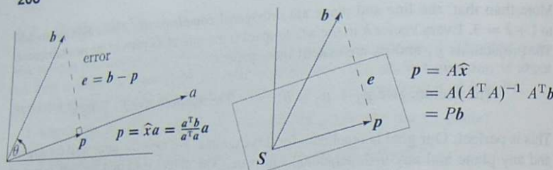
Figure 4.5: The projection p of b onto a line and onto S = \text{column space of } A .
