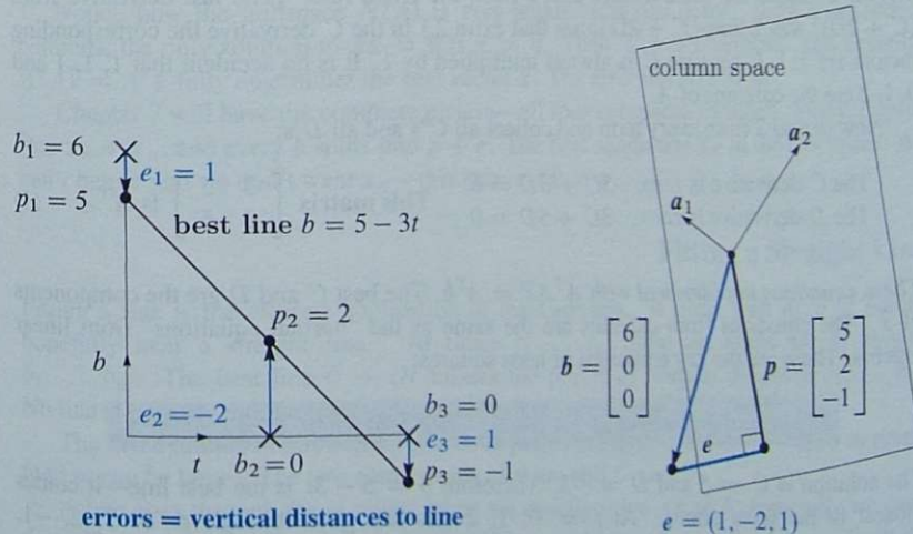
Figure 4.6: Best line and projection: Two pictures, same problem. The line has heights p = (5, 2, -1) with errors e = (1, -2, 1) . The equations A^T A\hat{x} = A^T b give \hat{x} = (5, -3) . The best line is b = 5 - 3t and the projection is p = 5a_1 - 3a_2 .
